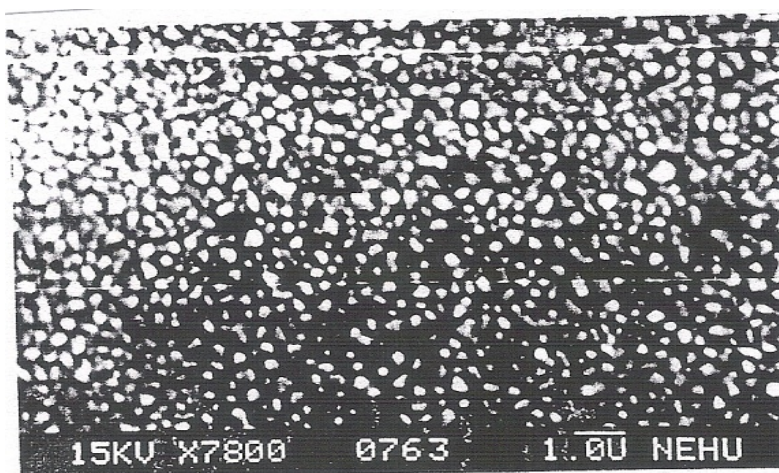
Fig. 2(d), SEM photograph of PbSe film ( x=1.0 )
