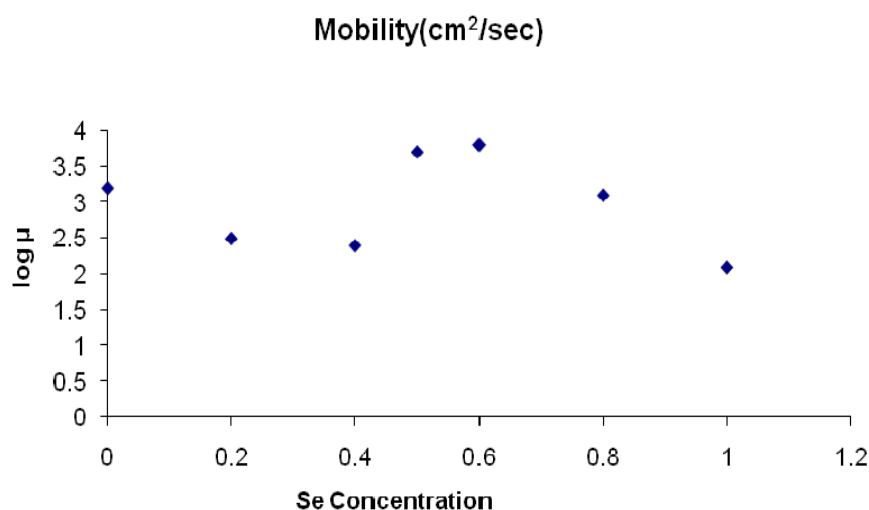
Fig. 5 Mobility
