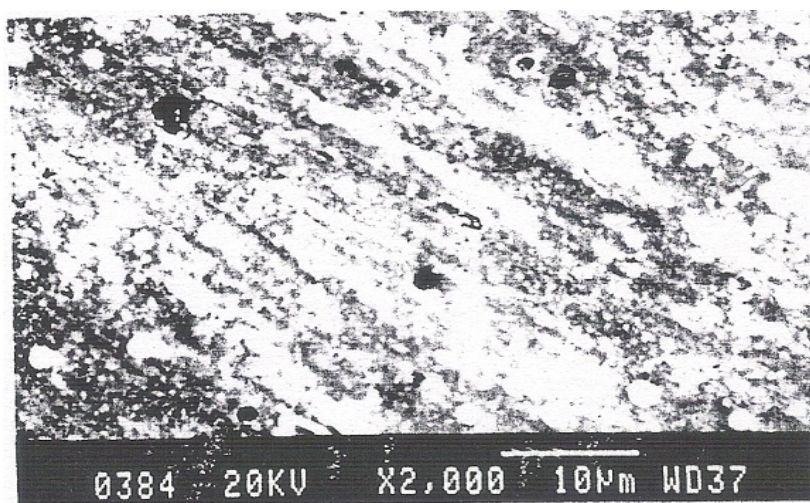
Fig. 2(c), SEM photograph of PbS.2Se.8 film ( x=0.8 )
