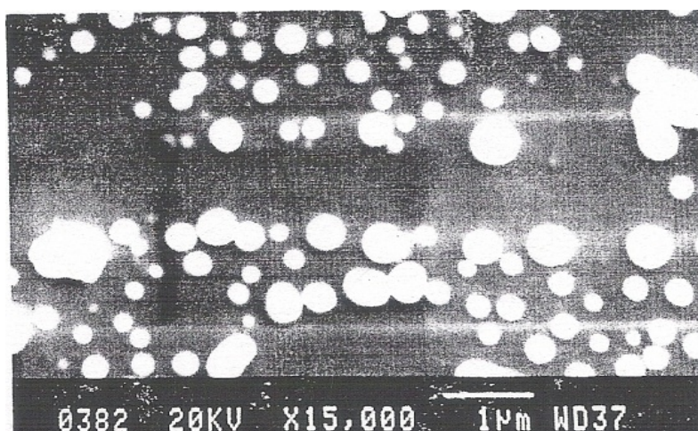
Fig. 2(b), SEM photograph of PbS.8Se.2 film ( x=0.2 )
