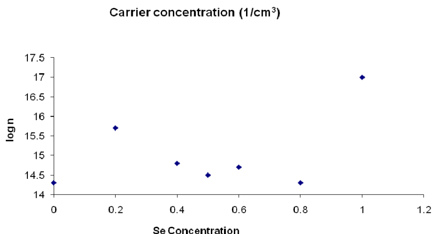
Fig. 4 Carrier concentration
