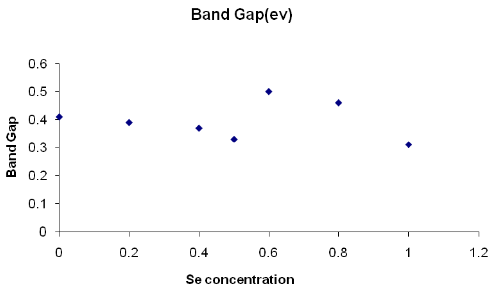
Fig. 6 Band gap.
