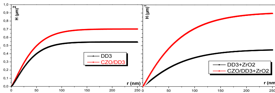
Fig. 5. Height–height correlation functions for Cu doped ZnO thin films deposited on DD3 and DD3+ \text{ZrO}_2 substrates
