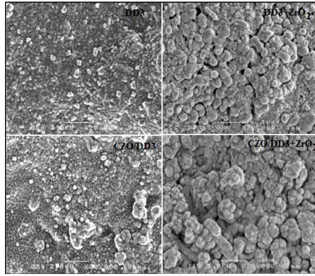
Fig. 4. SEM images of DD3 (a, b) and DD3+ \text{ZrO}_2 , (c, d) Cu doped ZnO.
