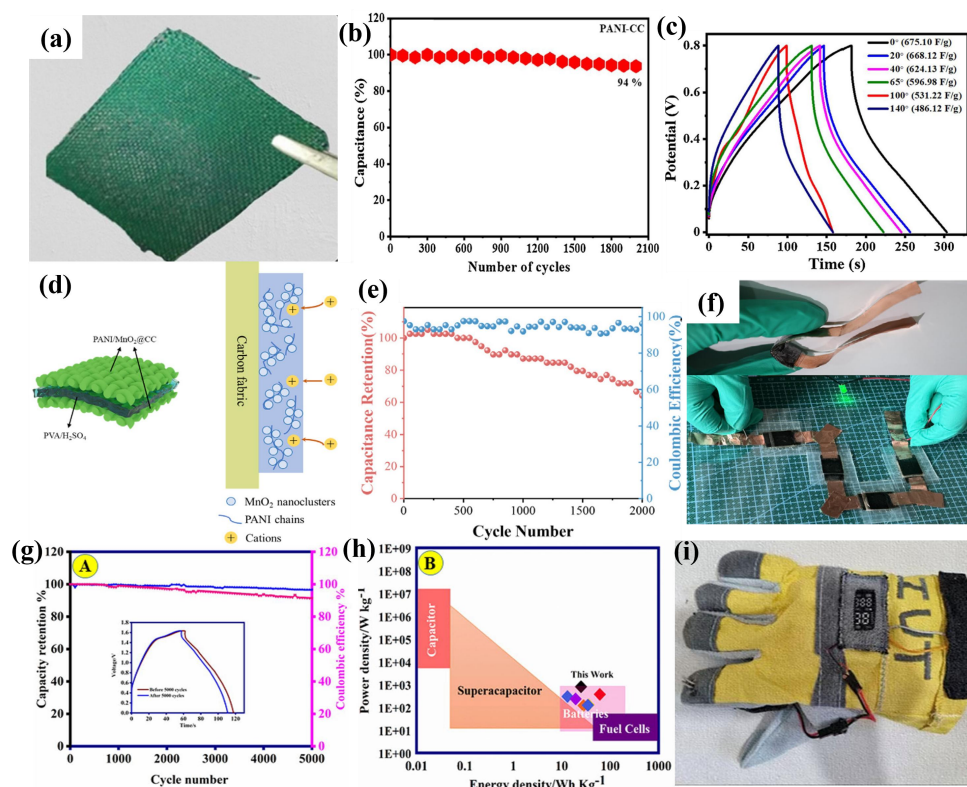
Figure 2. Different PANI-based flexible supercapacitors: (a) Digital images showing substrate after polymerization (PANI-CC), (b) Stability test up to 2000 GCD cycles for PANI-CC and (c) GCD (at 1 A/g) of PANI-CC flexible SC at each bending angle[37]; (d) Charge storage mechanism, (e) Cycling stability at 2.5 mA cm -2 of MnO 2 /PANI@CC and (f) Optical image of the supercapacitor under bending (top) and the symmetric supercapacitors with 4 in series lighting an LED (3 V) (bottom)[39]; (g) Ni-Co@PS-CC//AC device stability test at 9.0 A g -1 (the inset indicates the GCD of the primary electrode and after 5000 cycles), (h) Ragone plot of Ni-Co@PS-CC//AC device, (i) the digital image of a wearable supercapacitor that has been integrated into a glove for the purpose of powering an oximeter[41].
